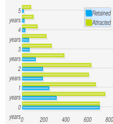
OpenStack
